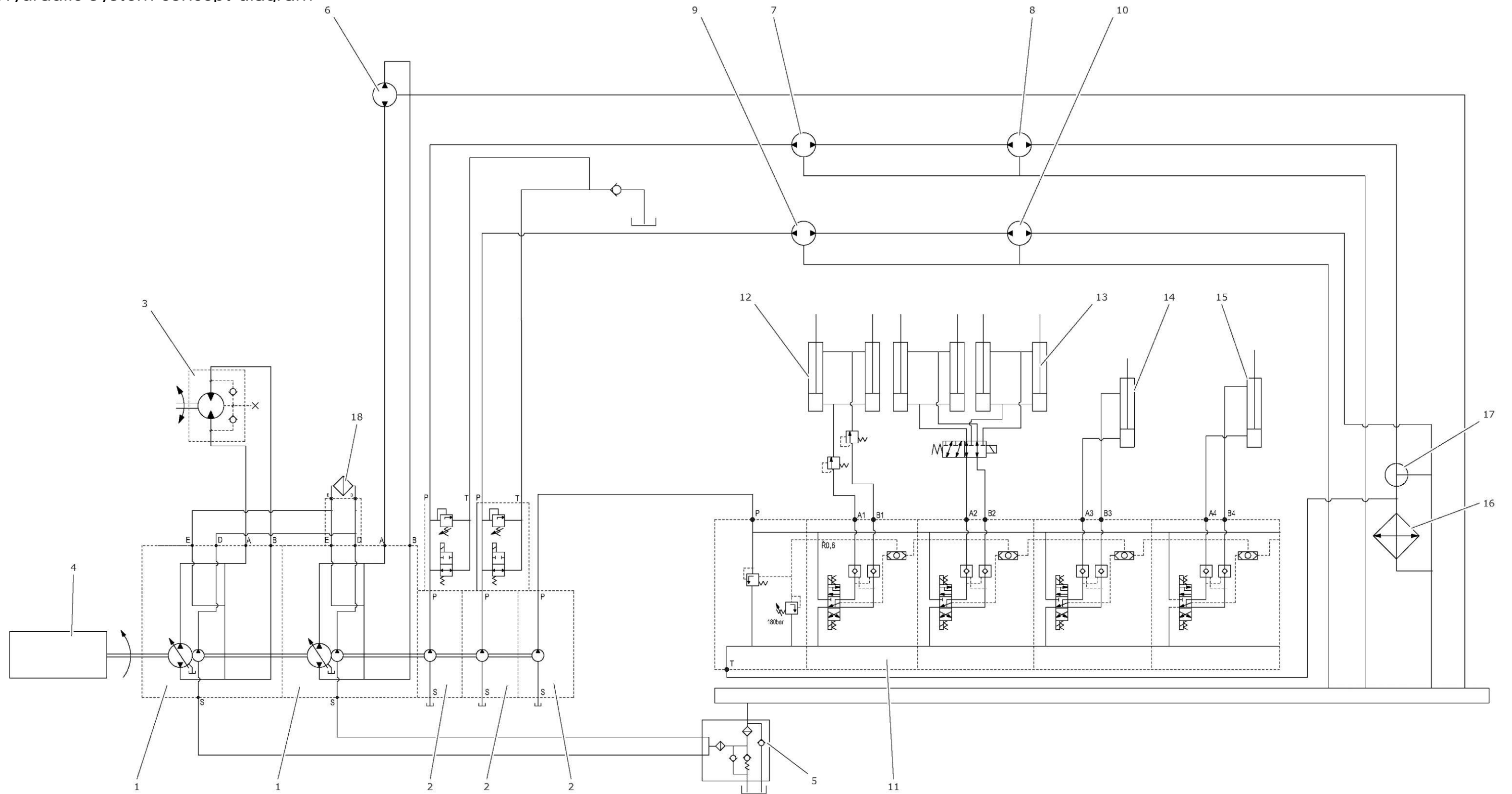
Hydraulic system concept diagram
