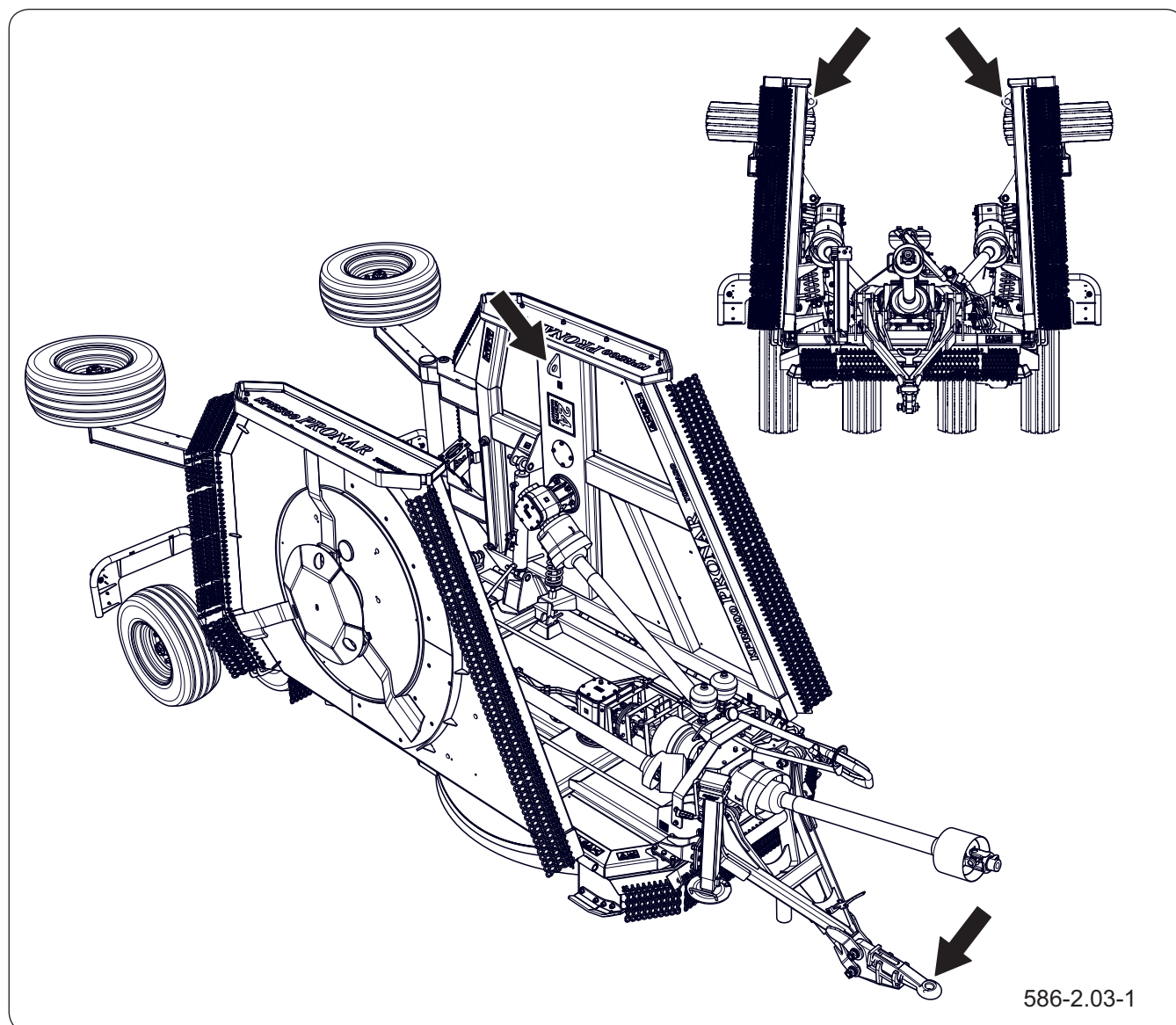
Figure 2.6 Points de fixation
