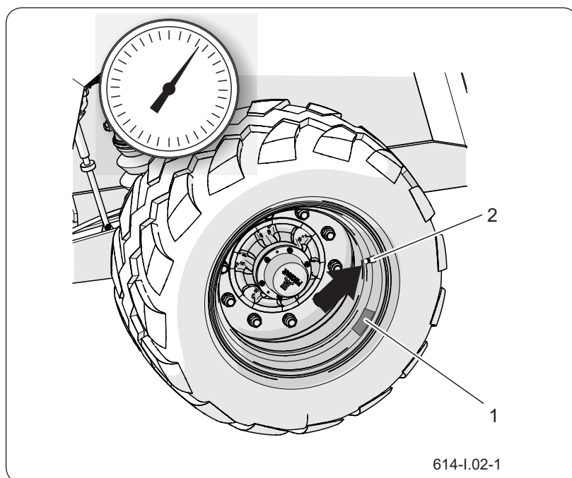
Figure 6.2 Roue de machine (1) autocollant (2) vanne
