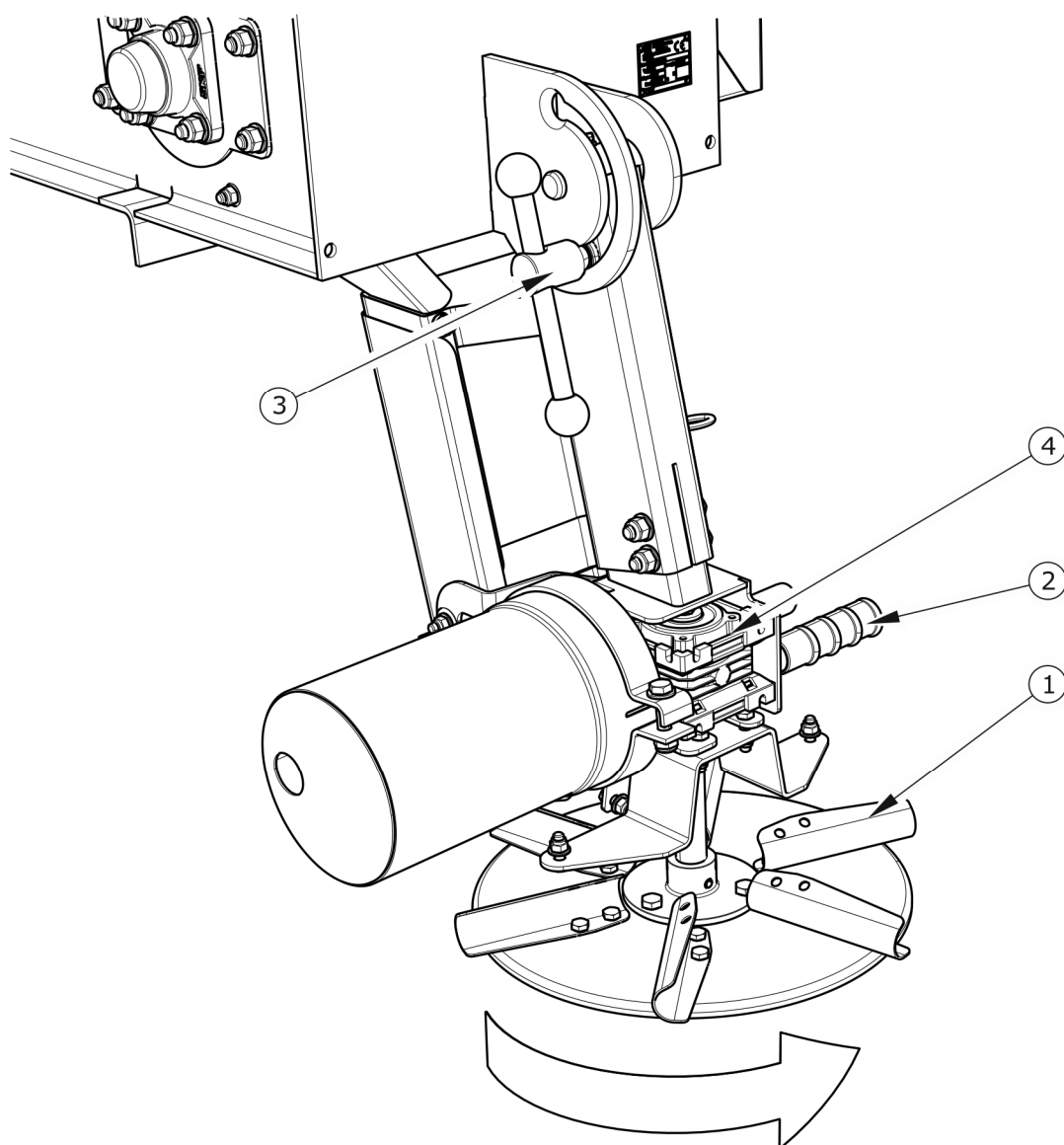
FIGUR 3.3 Spredtheadapter
